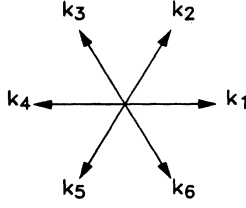
FIG. 3. Arrangement of the six wave vectors forming regular hexagons.
